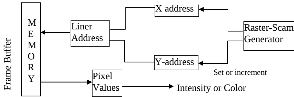
Figure: Organization of Video Controller.
